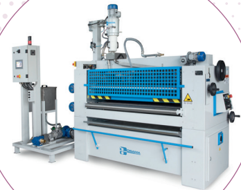
S4R + mixer
